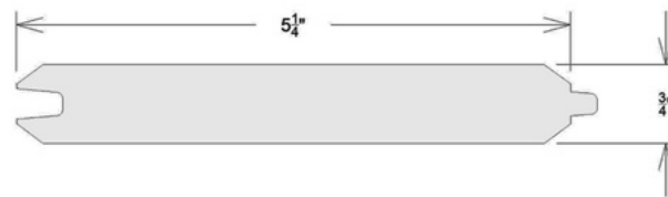
"V" JOINT MISC 007 (5 1/4" & 7 1/4")
