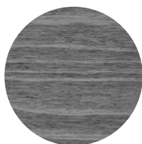
Cyclone
