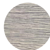
Tephra
